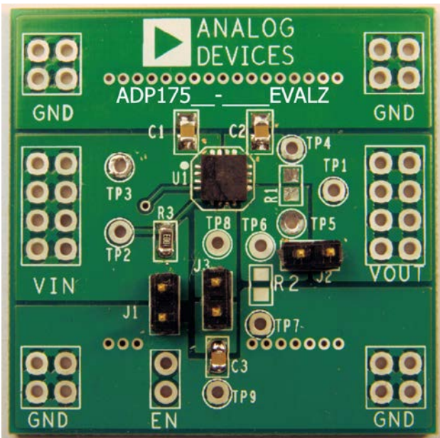
Figure 46. Evaluation Board
